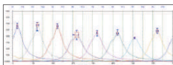
Engine Power Cylinder Parade
